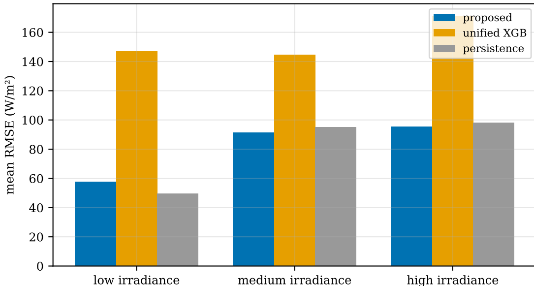
Conditional error by irradiance regime (all 42 pairs)
