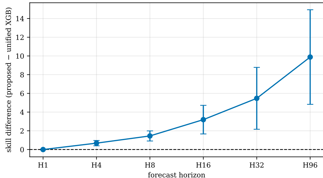
Paired skill advantage with 95% CI (from existing predictions)
