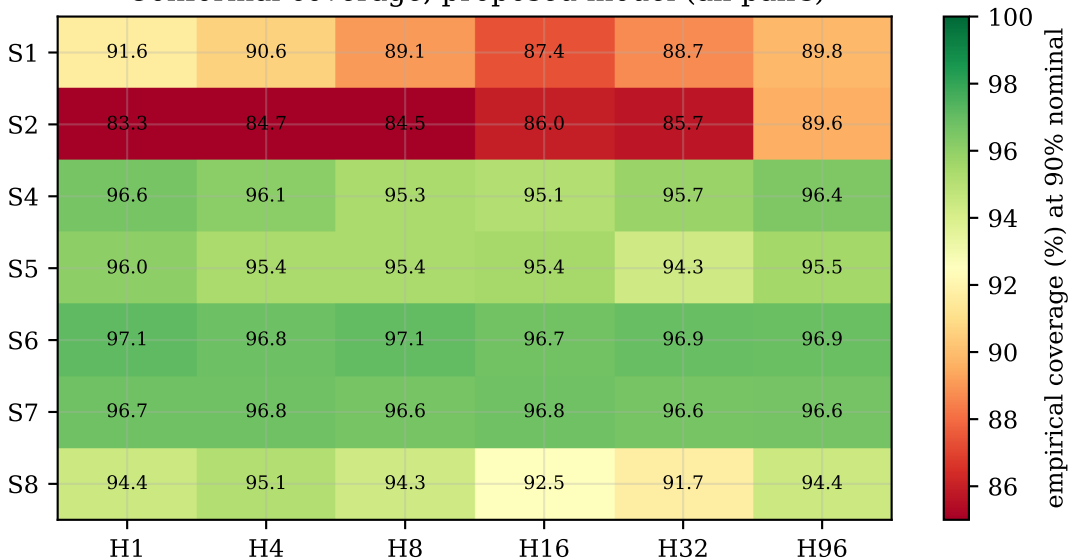
Conformal coverage, proposed model (all pairs)
