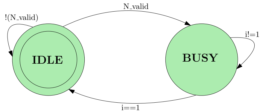
Control FSM
