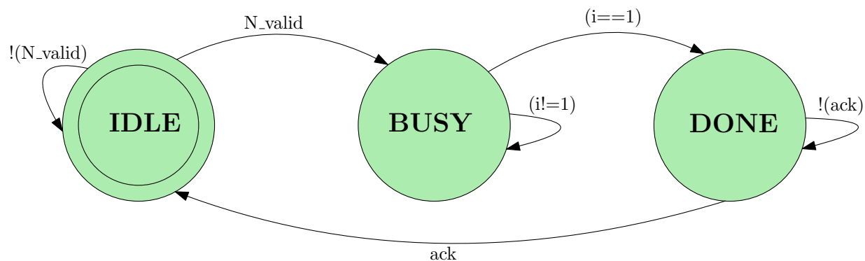
Control FSM
