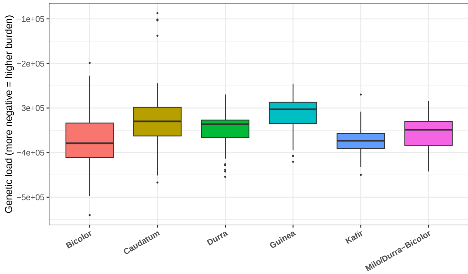
SAP Genetic Load (miss50) – 5% cutoff
