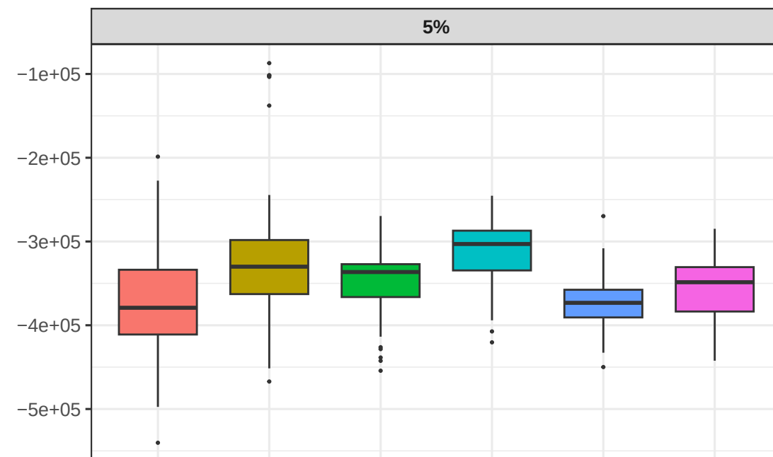
SAP Genetic Load by Race Across Cutoffs (miss50)
