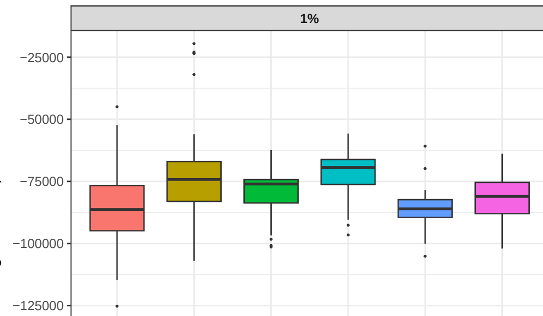
SAP Genetic Load by Race Across Cutoffs (miss50)
