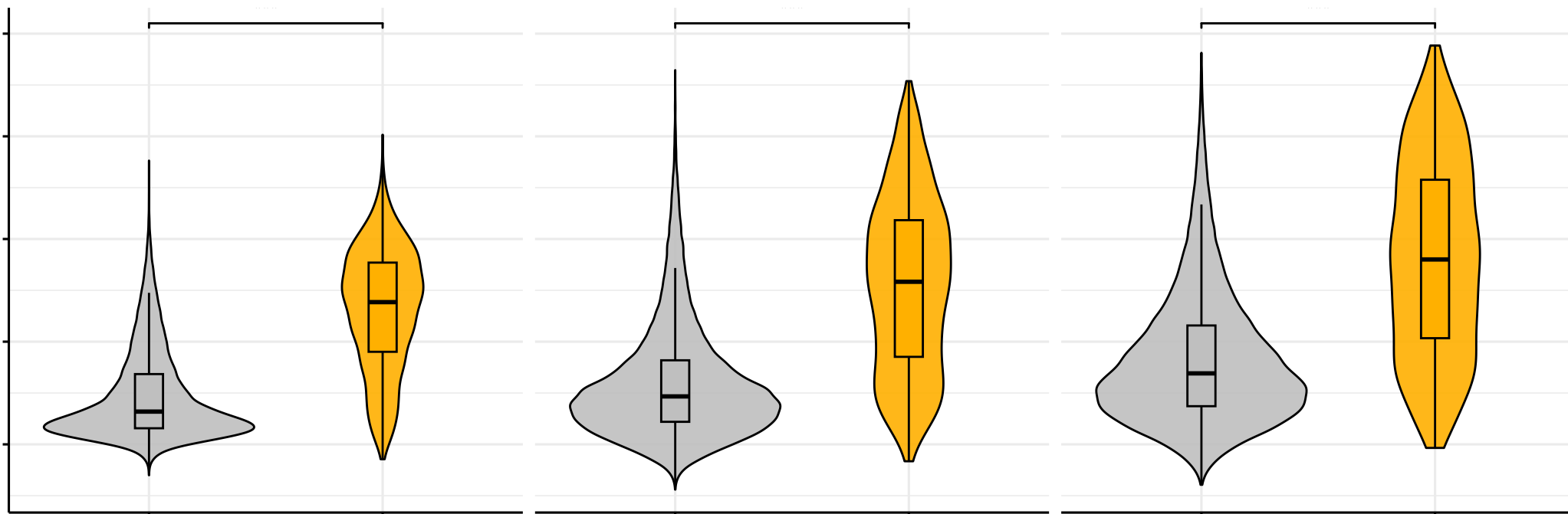
Nucleotide diversity ( \pi )
