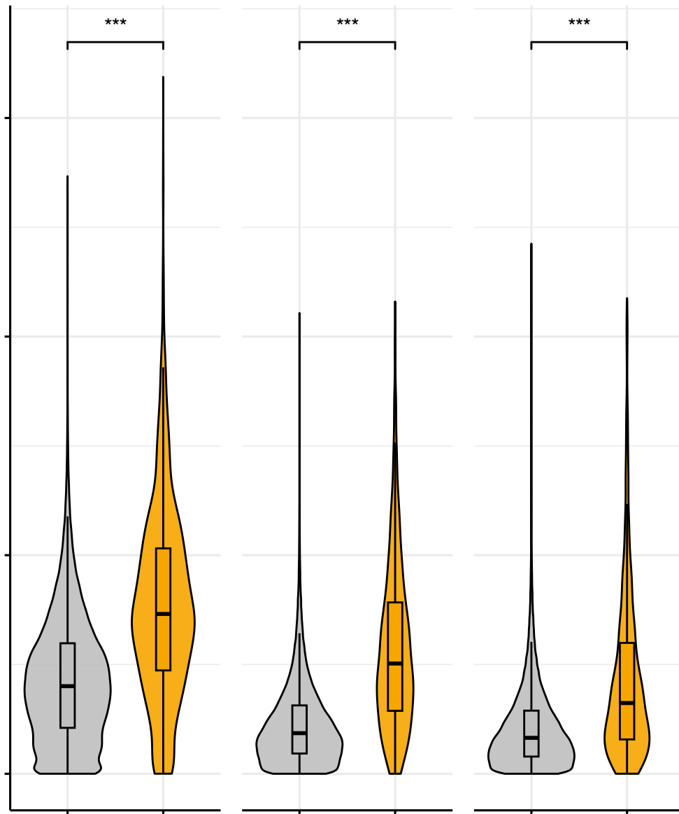
Nucleotide diversity ( \pi )
