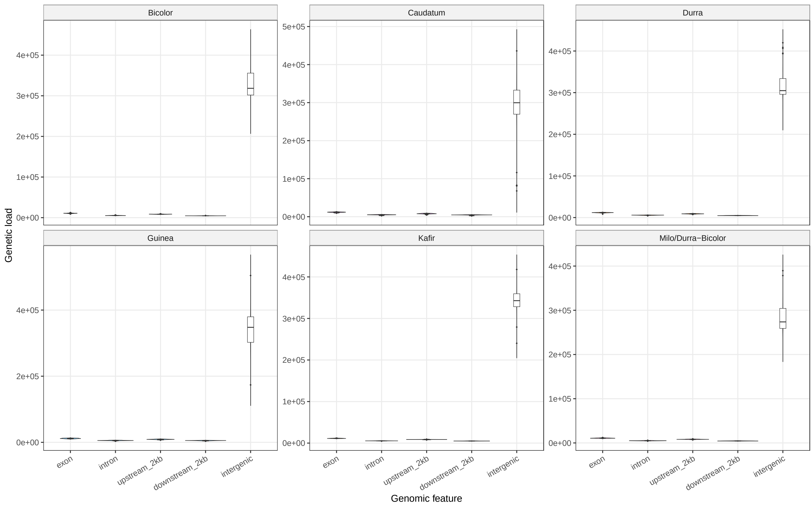
SAP top 5% feature-level genetic load by race
