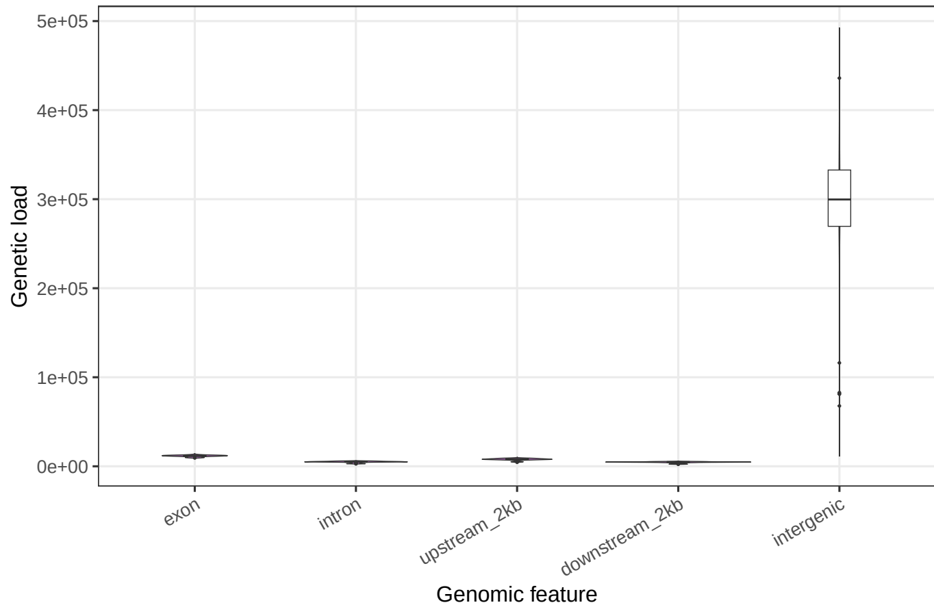
SAP top 5% feature-level load: Caudatum
