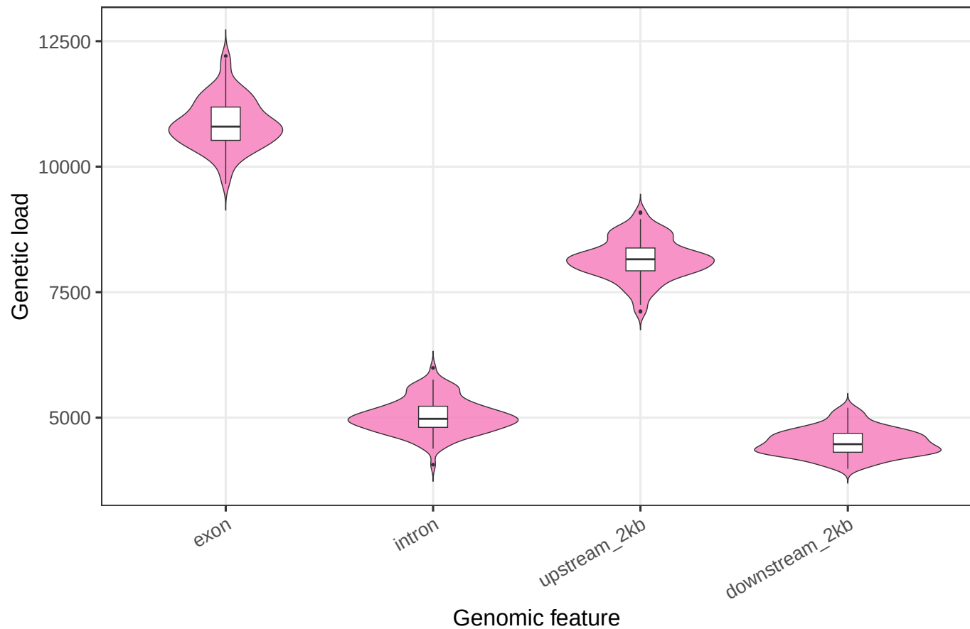
SAP top 5% feature-level load (no intergenic): Milo/Durra-Bicolor
