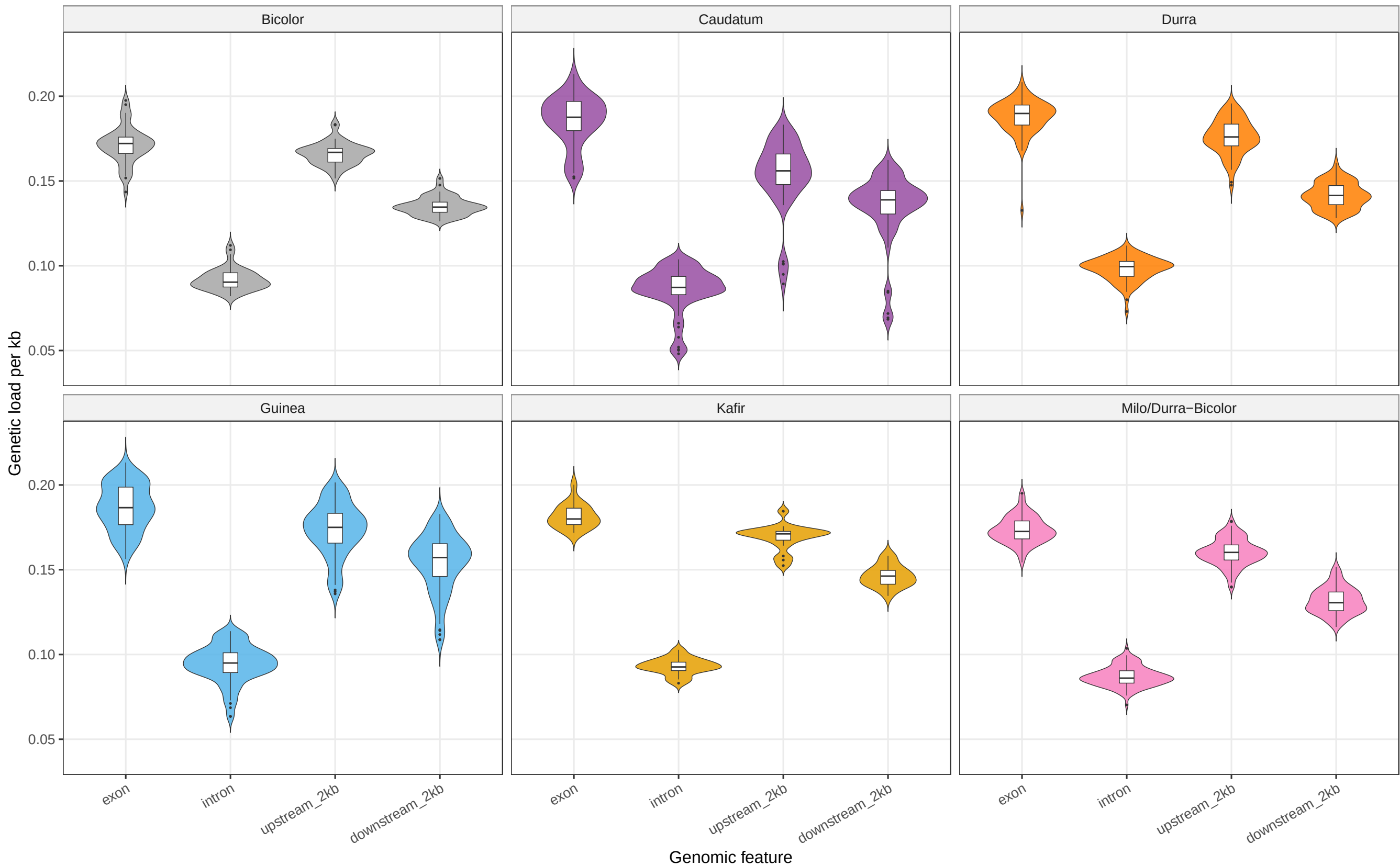
SAP top 5% feature-level genetic load per kb by race (no intergenic)
