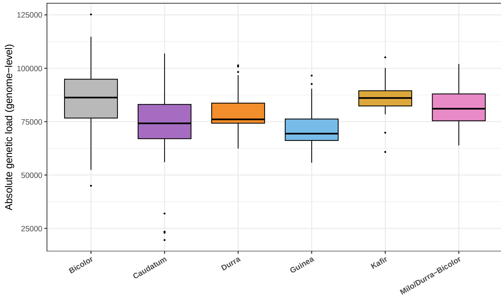
SAP top 1% (genome-level, miss50)
