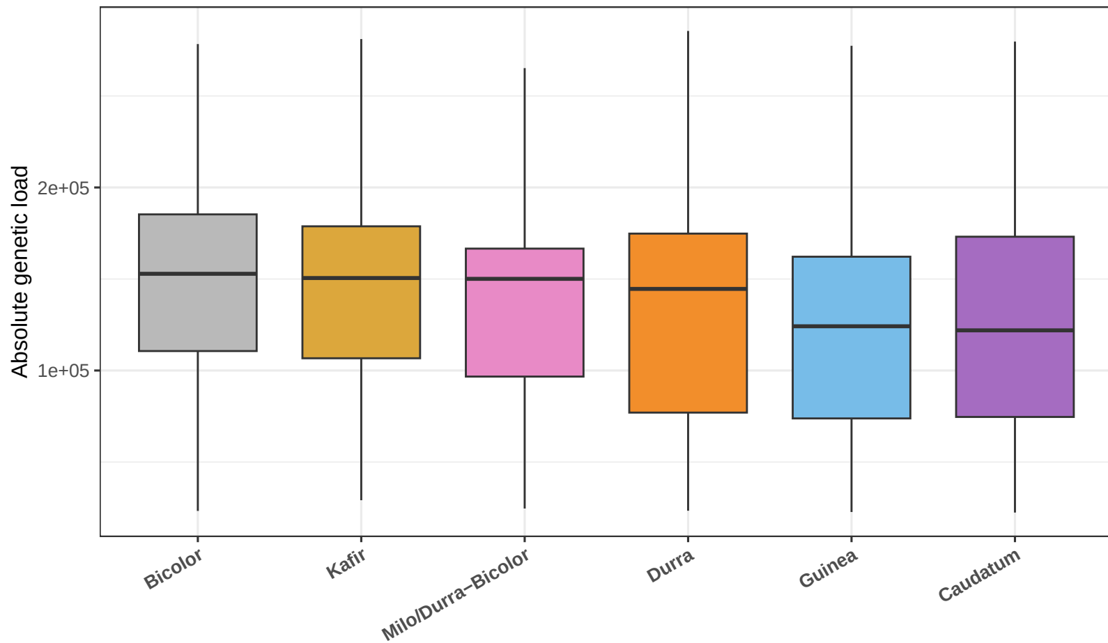
SAP chr-level absolute genetic load by race (25%, miss50)
