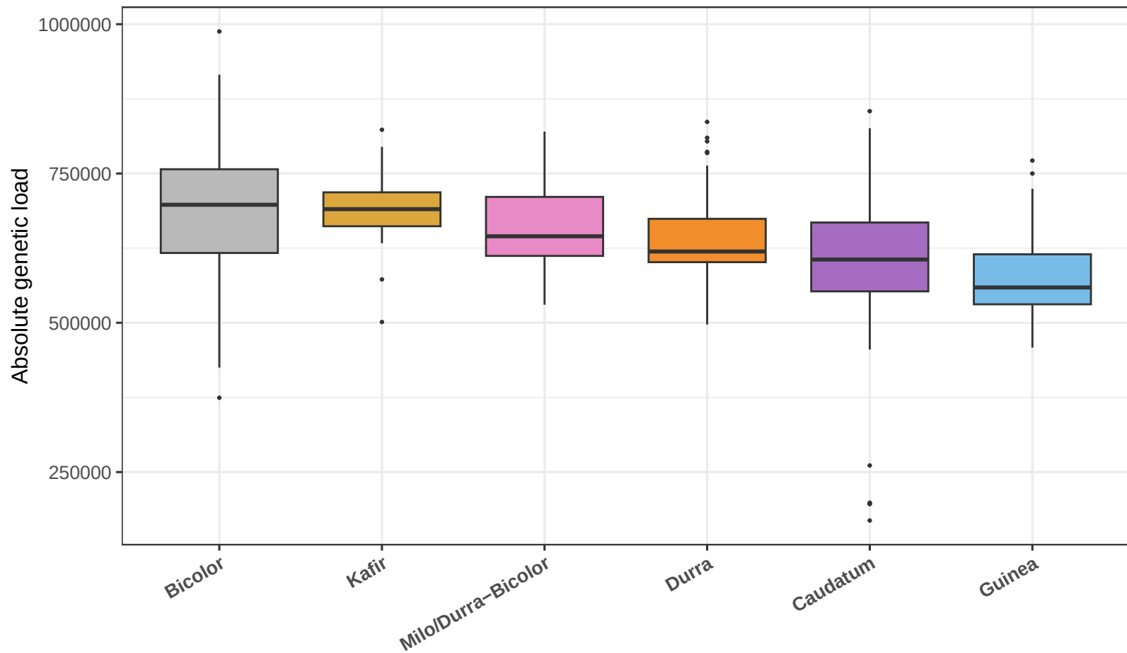
SAP genome-level (sum chr) absolute load by race (10%, miss50)
