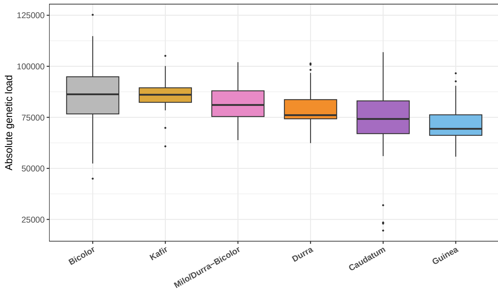
SAP genome-level (sum chr) absolute load by race (1%, miss50)
