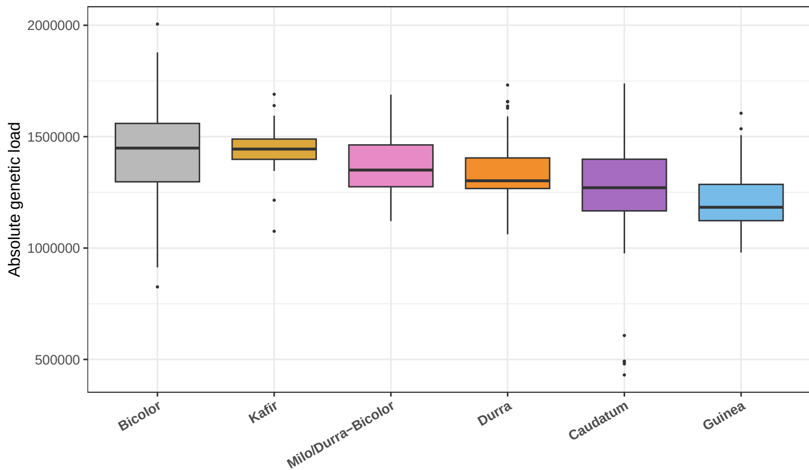
SAP genome-level (sum chr) absolute load by race (25%, miss50)
