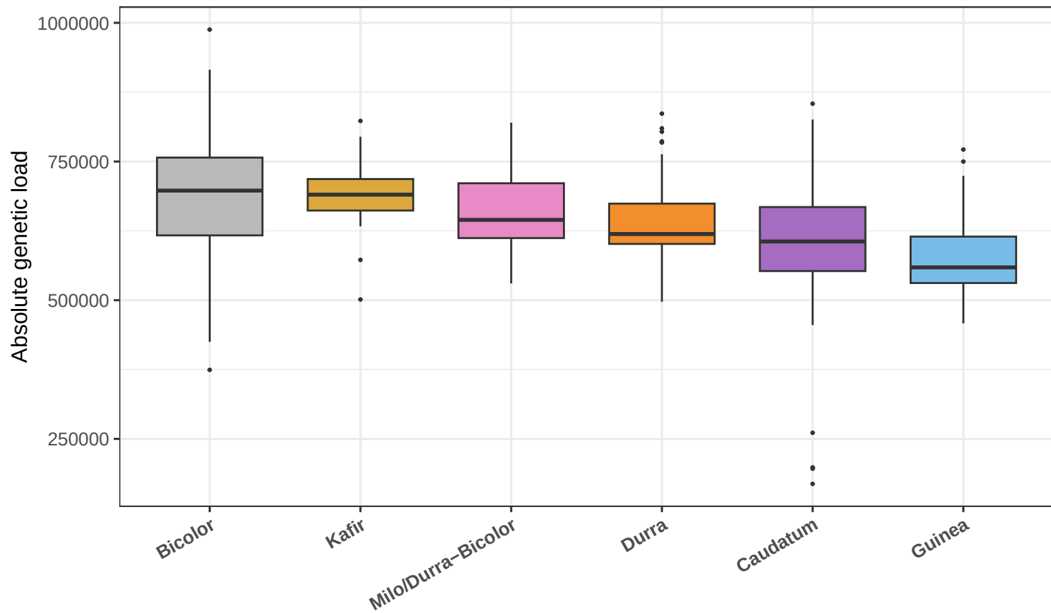
SAP Absolute Genetic Load (miss50) – 10% cutoff
