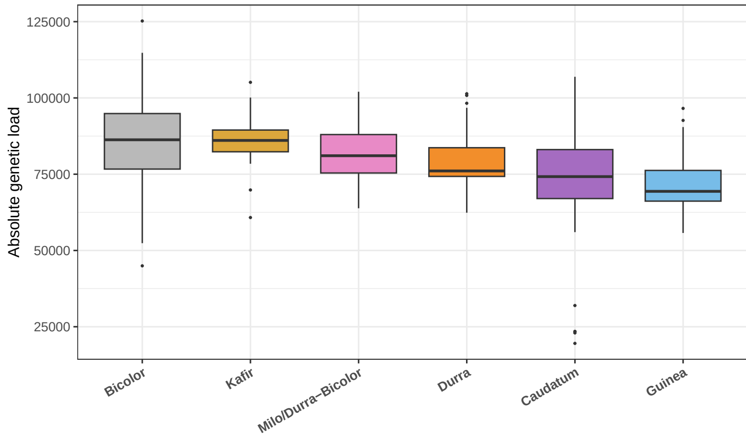
SAP Absolute Genetic Load (miss50) – 1% cutoff
