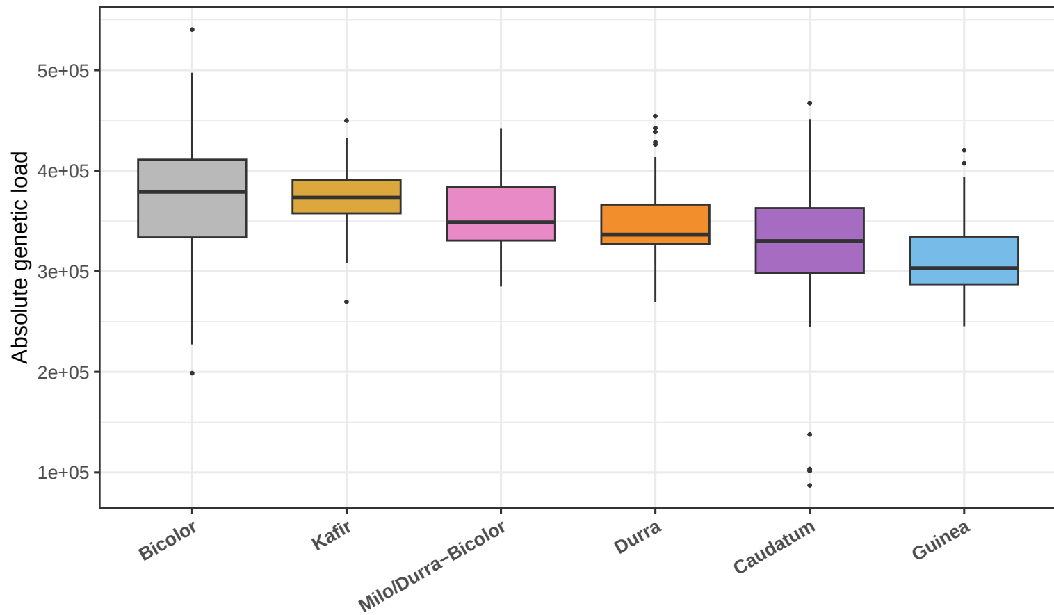
SAP Absolute Genetic Load (miss50) – 5% cutoff
