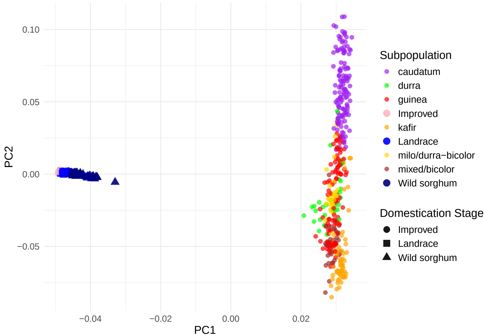
PCA of Merged Sorghum Datasets
