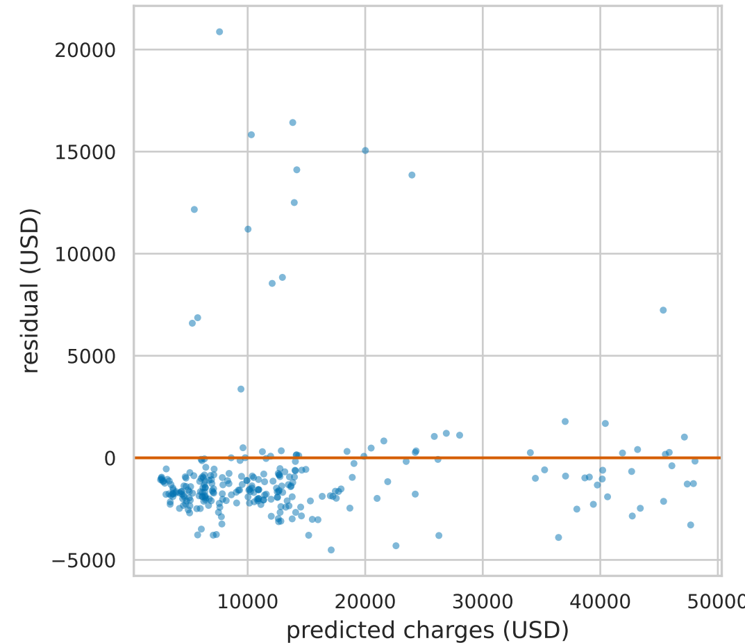
(e) Residuals vs Fitted (GB)
