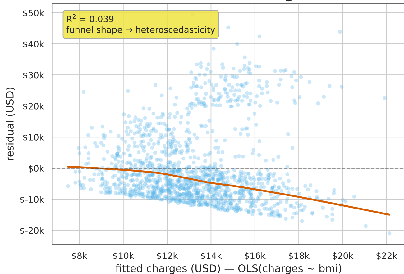
Residuals vs fitted — charges ~ bmi
