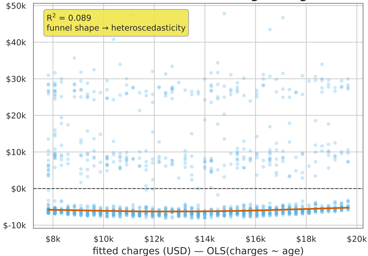
Residuals vs fitted — charges ~ age
