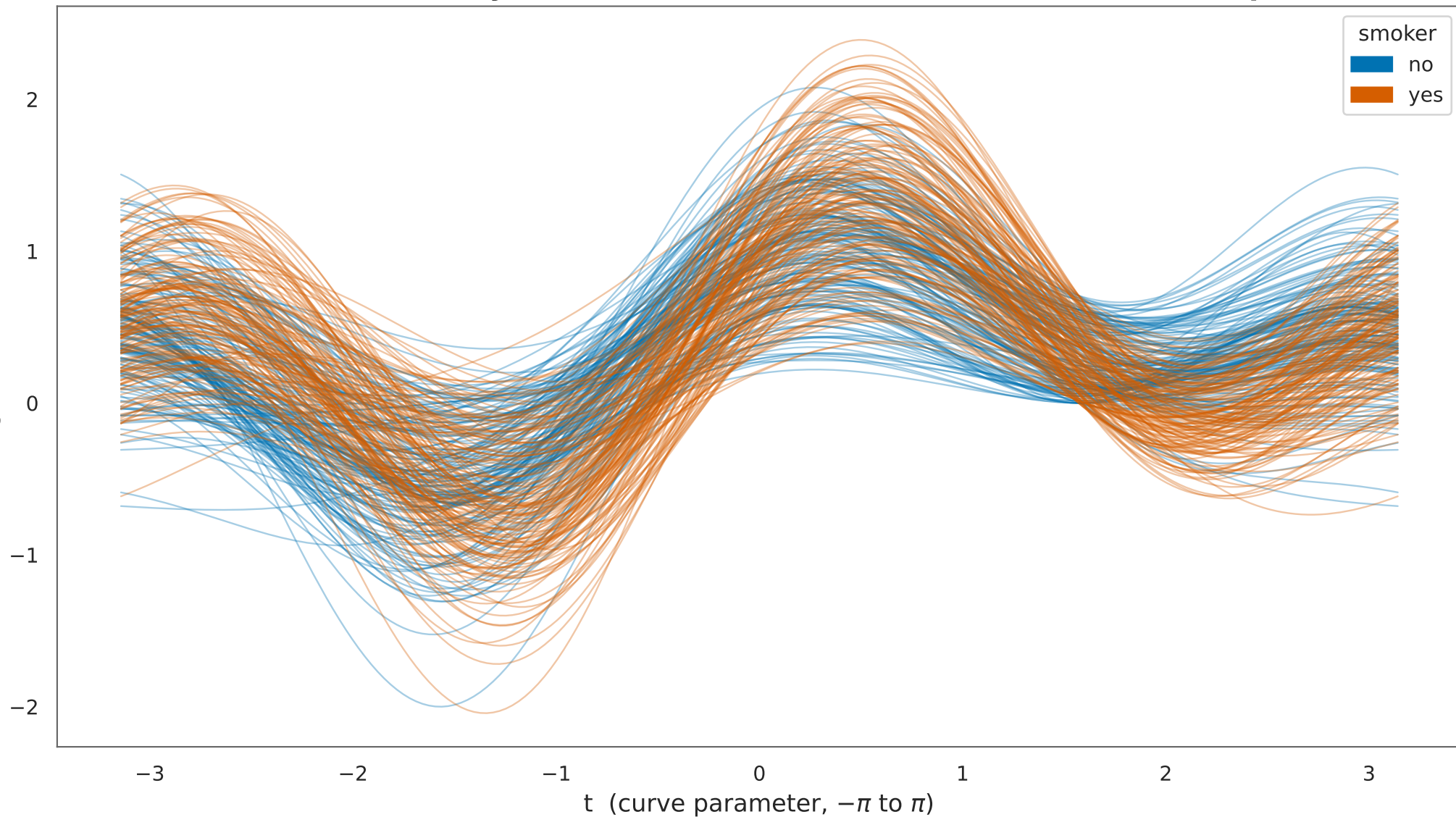
Andrews curves by smoker — normalized features (~300-row sample)
