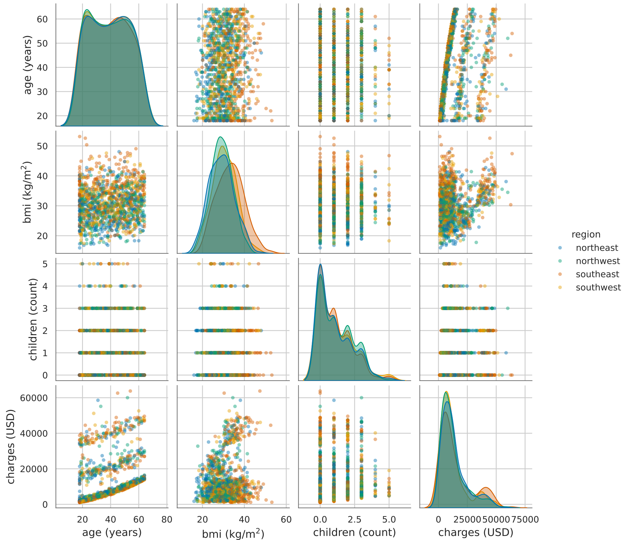
Scatter-matrix of numeric features — colored by region
