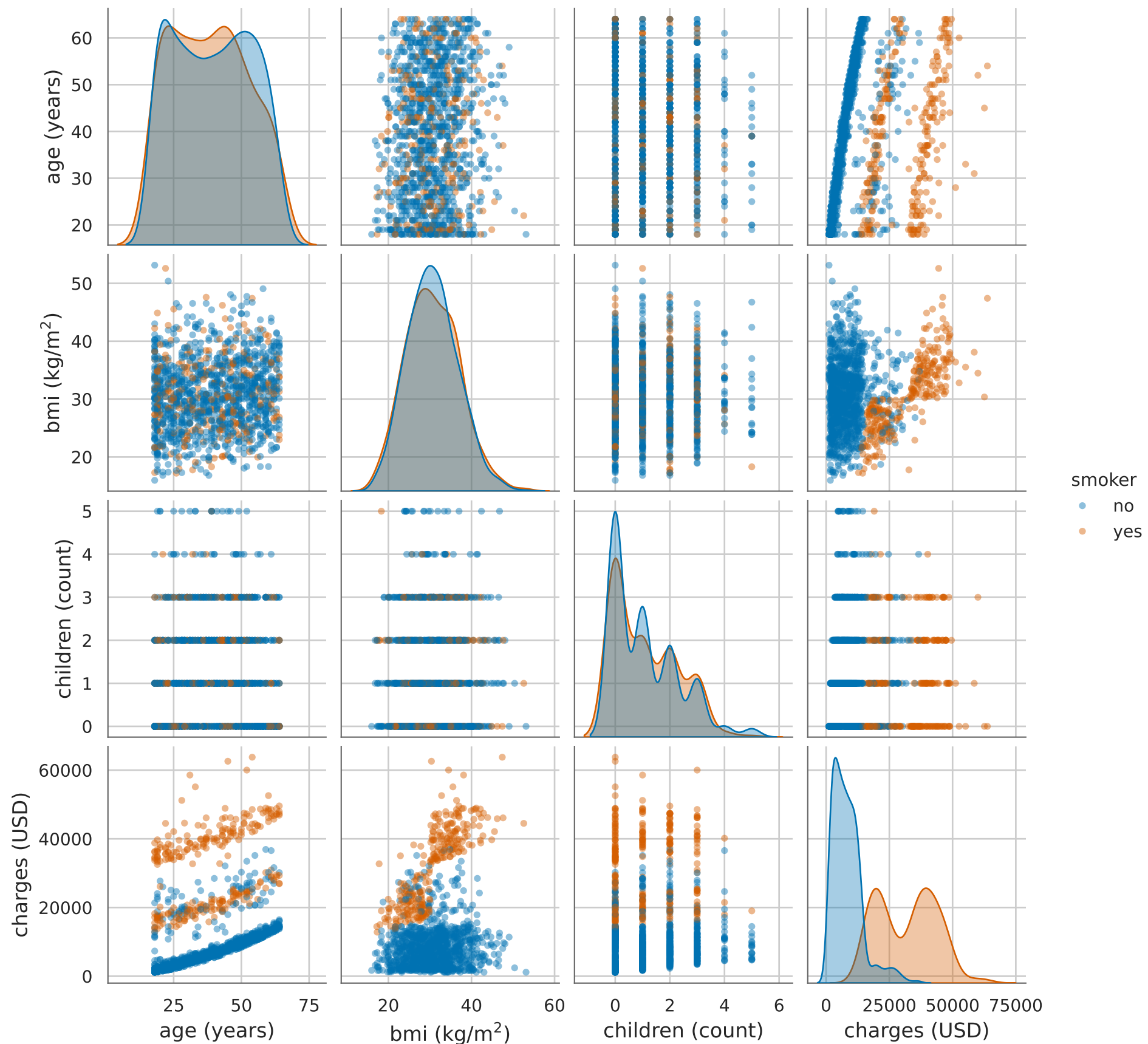
Scatter-matrix of numeric features — colored by smoker
