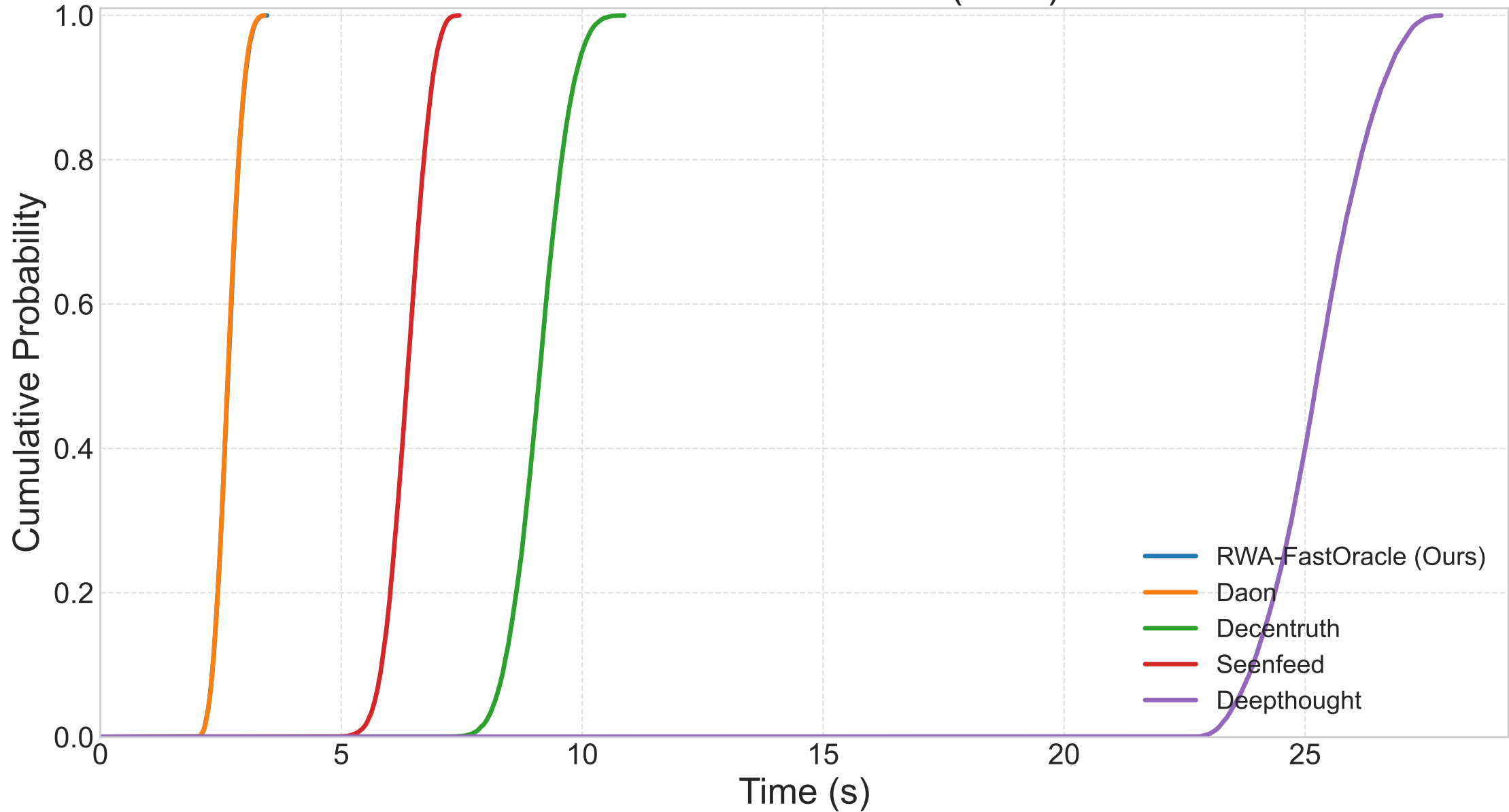
Consensus Time CDF (POS)
