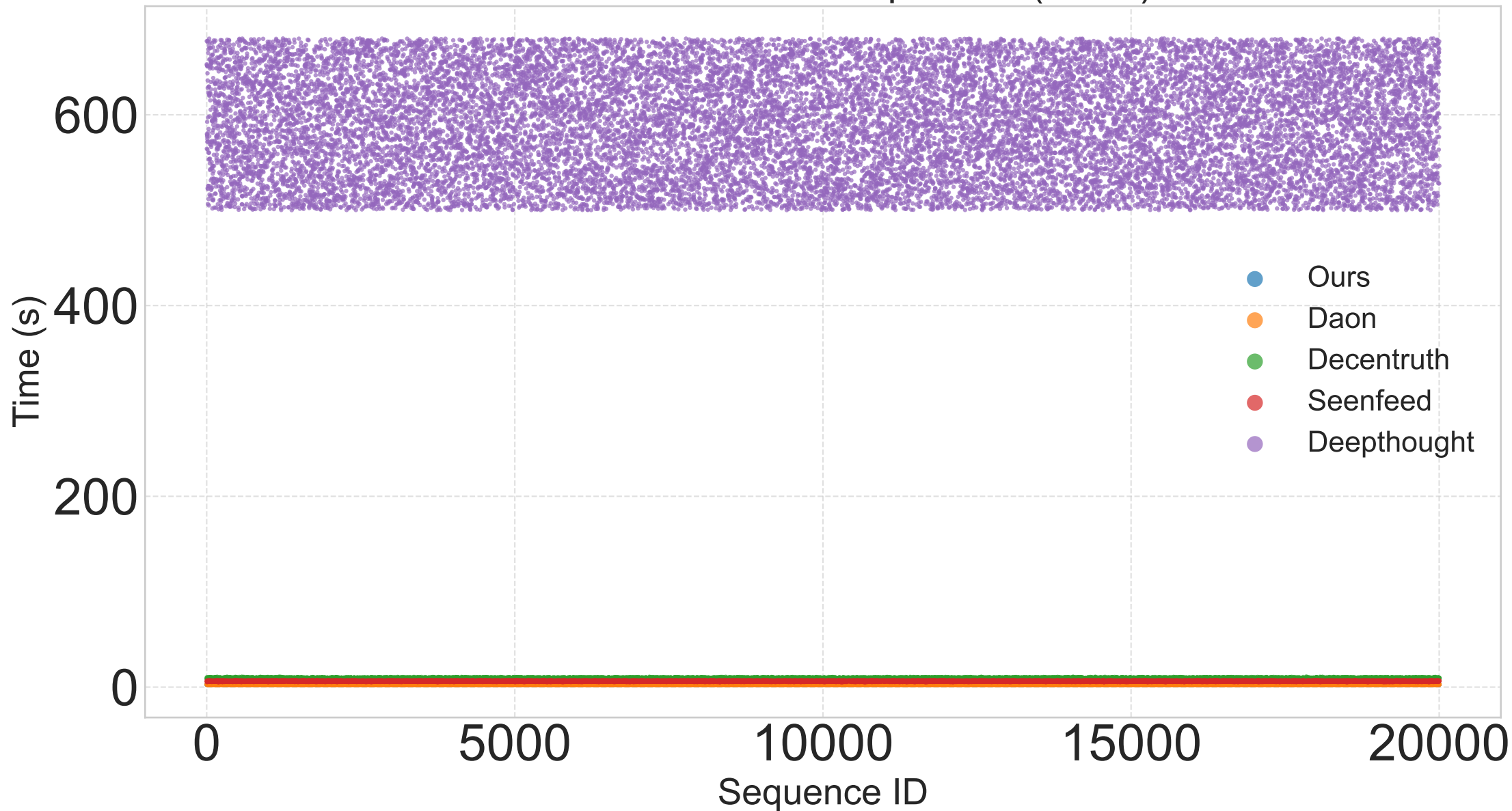
Consensus Time Comparison (POW)
