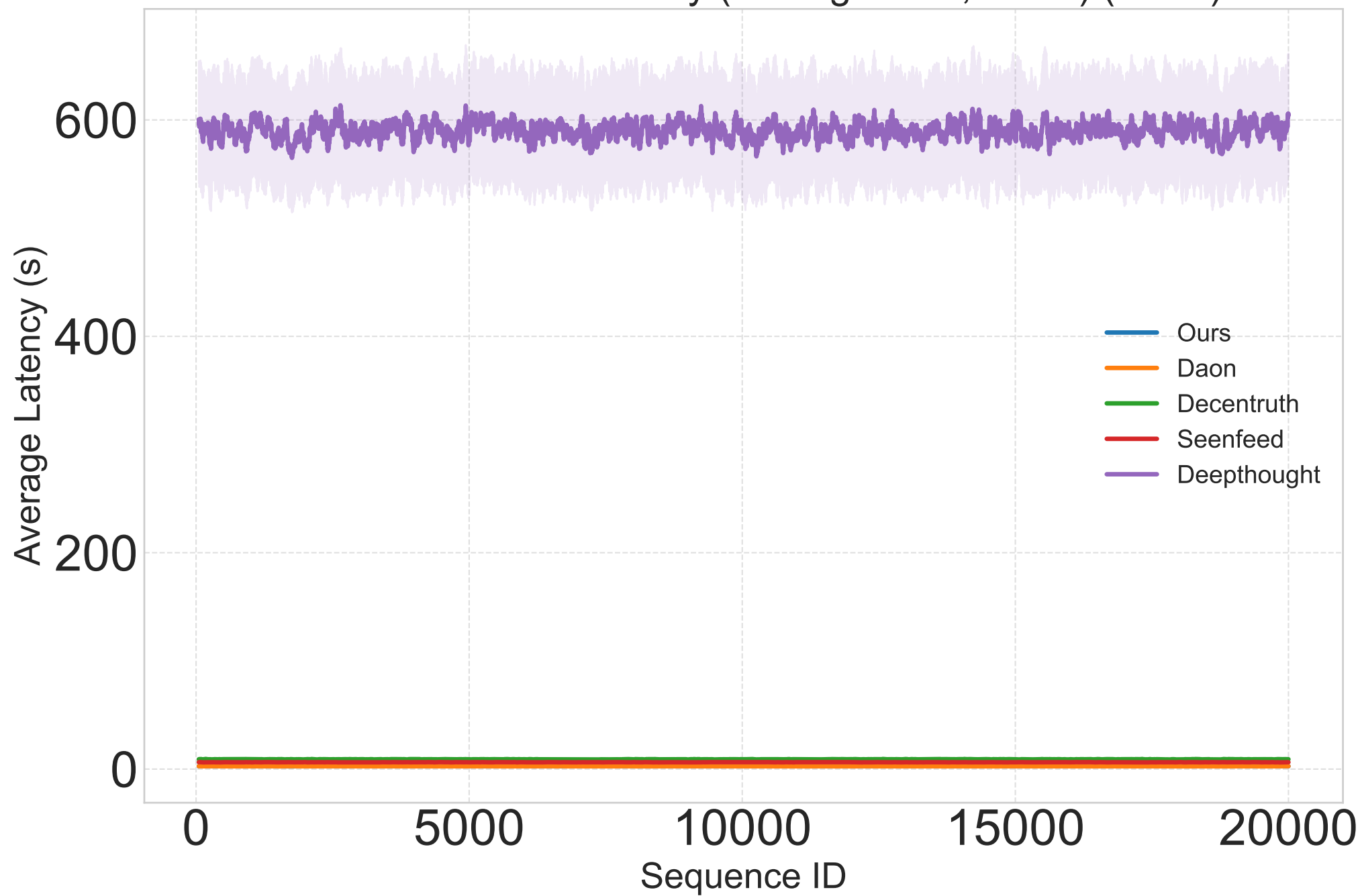
Consensus Time Stability (Rolling Mean, w=50) (POW)
