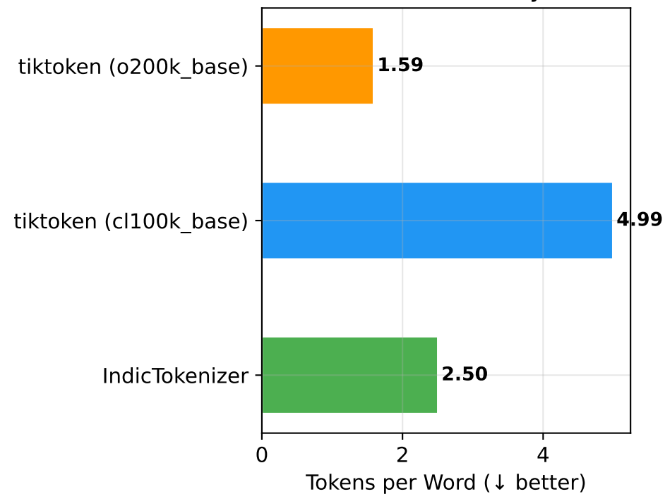
Token Efficiency
