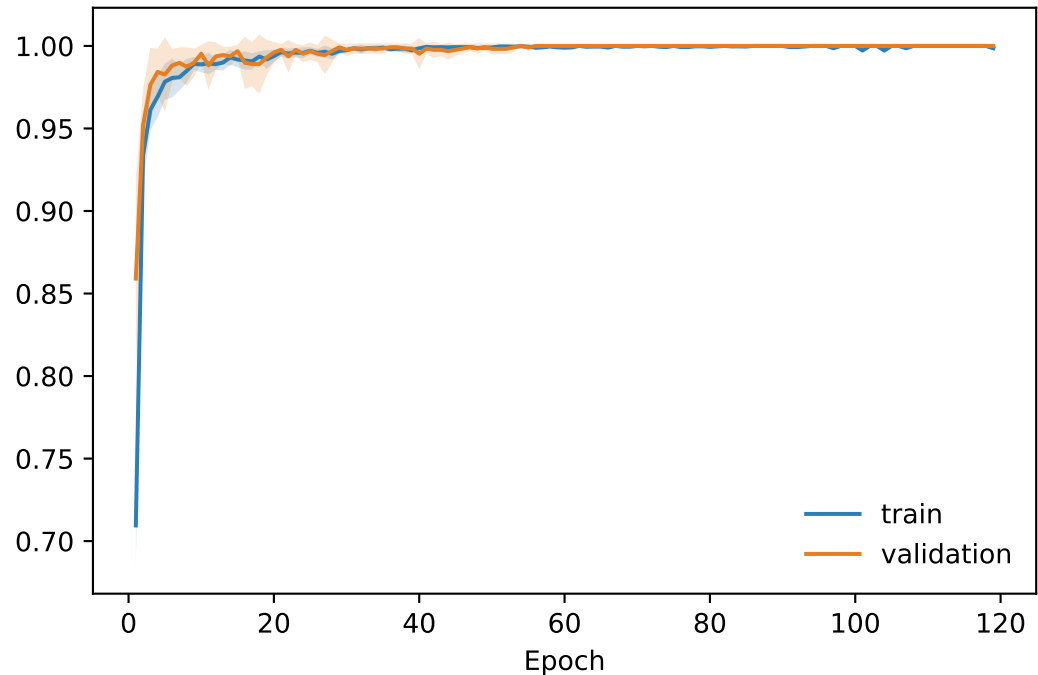
CNN accuracy (mean \pm SD, 10 initialisations)
