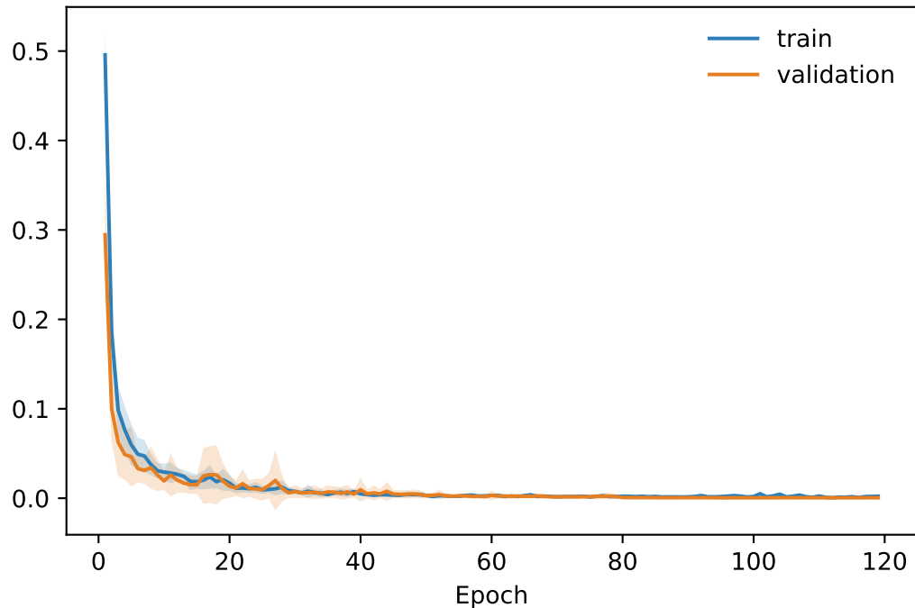
CNN loss (mean \pm SD, 10 initialisations)
