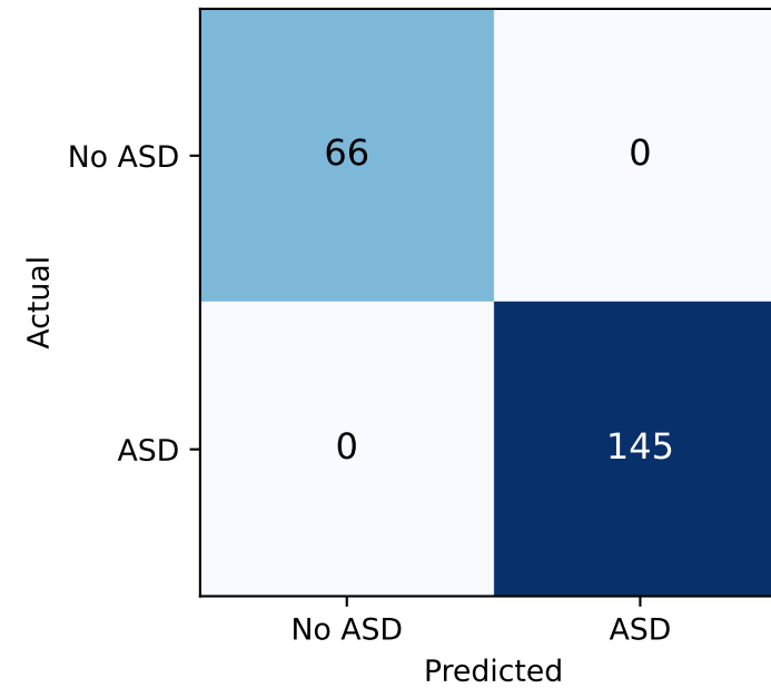
Gradient Boosting
