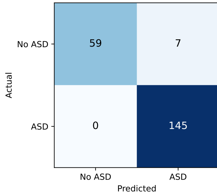
Random Forest
