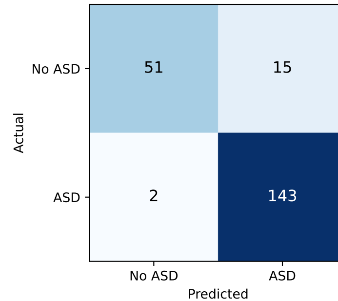
Naive Bayes
