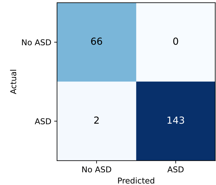
1D CNN
