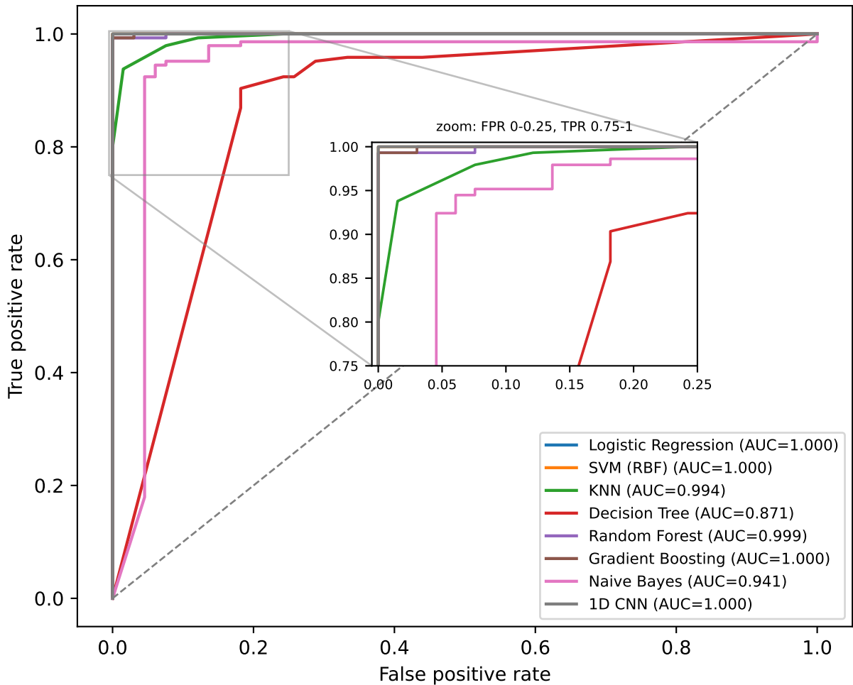
ROC curves - test set
