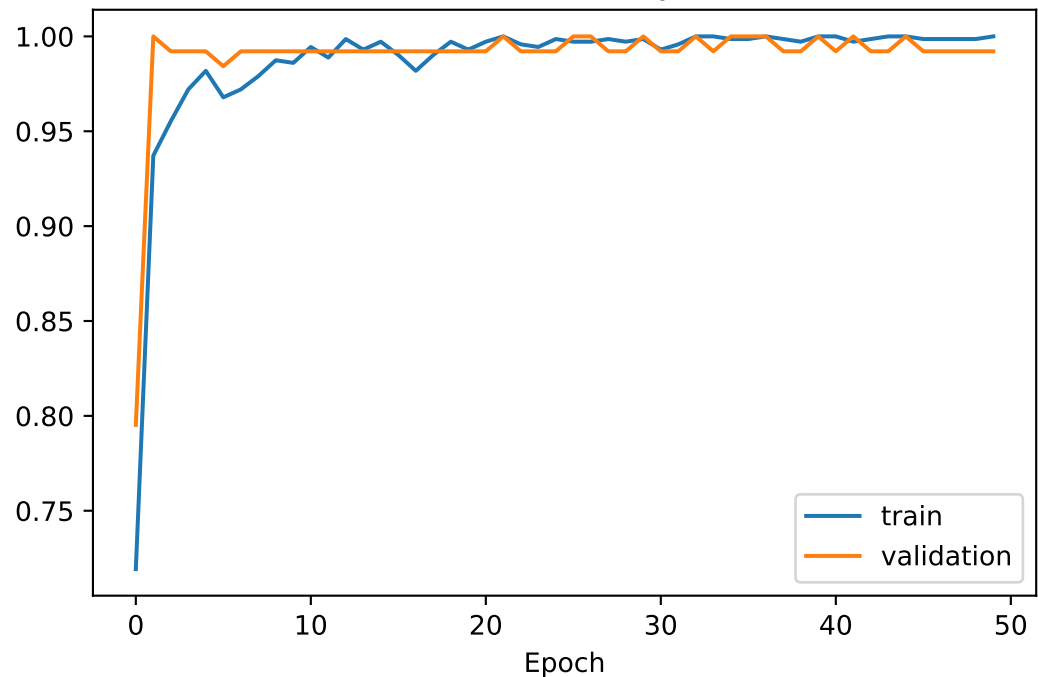
CNN accuracy
