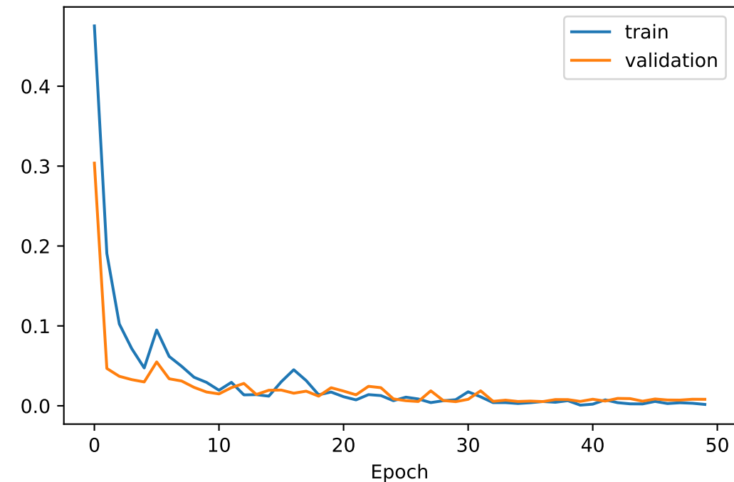
CNN loss
