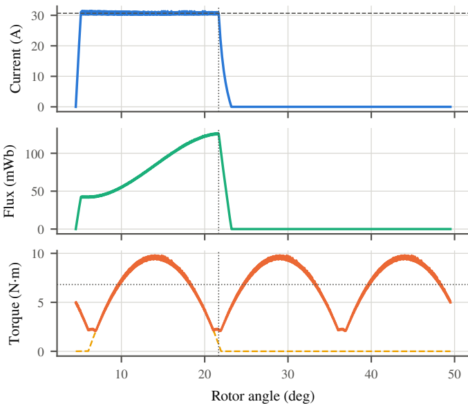
Current chopping: 80 r/min, \theta_{on}=4.5^\circ , \theta_{off}=21.7^\circ
