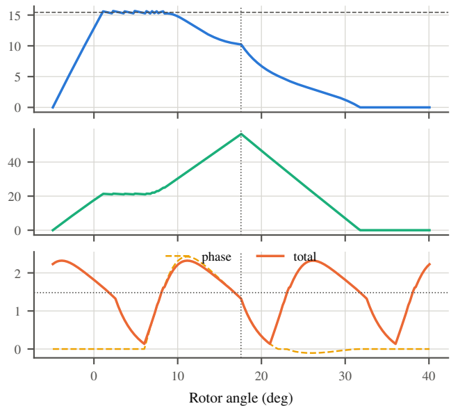
Rated, single pulse: 1608 r/min, \theta_{on}=-4.9^\circ , \theta_{off}=17.6^\circ
