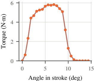
(a) CCC, 200 r/min, 3 N·m
