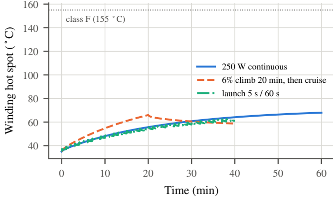
Fig. 11. Predicted winding hot-spot temperature ( h = 25 \text{ W/m}^2\text{K} , 35^\circ\text{C} ambient).
