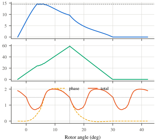
Rated, single pulse: 1608 r/min, \theta_{on}=-2.9^\circ , \theta_{off}=15.1^\circ
