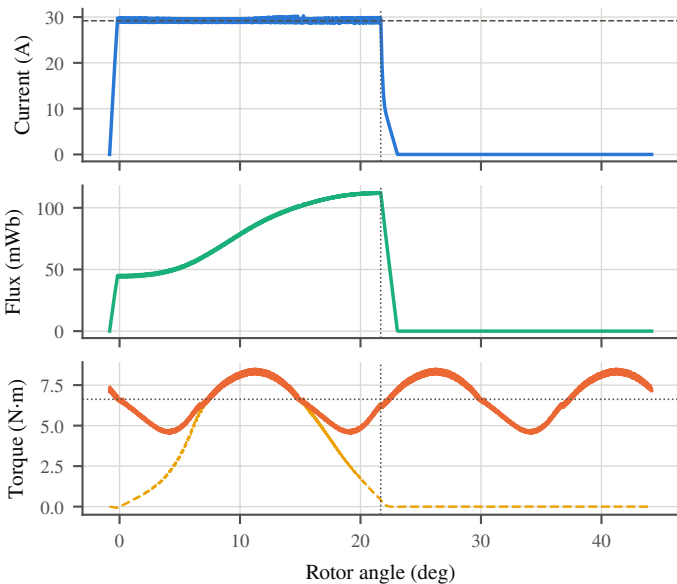
Current chopping: 80 r/min, \theta_{on}=-0.8^\circ , \theta_{off}=21.7^\circ
