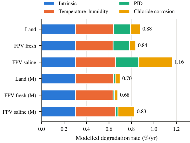
Fig. 7. Modelled module degradation rate by mechanism (baseline). (M): PID-resistant and salt-mist-hardened modules with the assumed factors of Table V.
