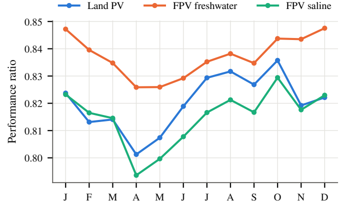
Fig. 5. Monthly performance ratio (baseline).
