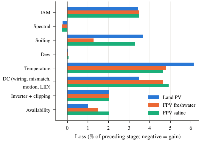
Fig. 4. Year-1 sequential loss breakdown (baseline). Negative values are gains.
