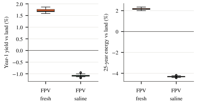
Fig. 11. Weather variability only: distribution over 20 synthetic years of the FPV year-1 yield and 25-year energy relative to land PV.
