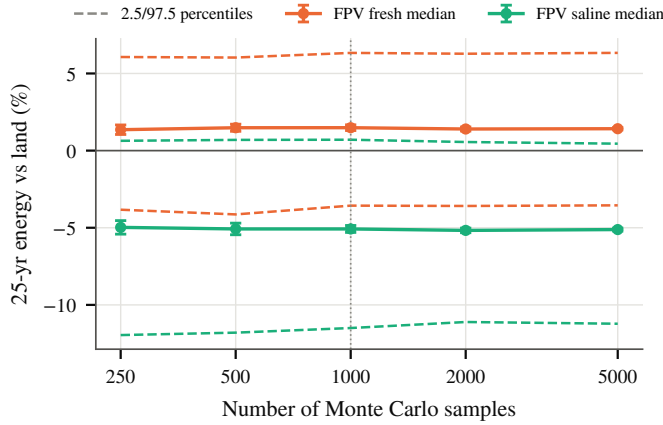
Fig. 13. Convergence of the Monte Carlo median (with \pm 1.96 bootstrap SE) and 95% bounds of the 25-year energy difference relative to land PV on nested subsets of one 5,000-sample run. The dotted line marks the 1,000 samples used in the paper.
