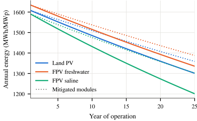
Fig. 8. Annual energy over 25 years (baseline). Dotted lines: PID-resistant and salt-mist-hardened modules (M).
