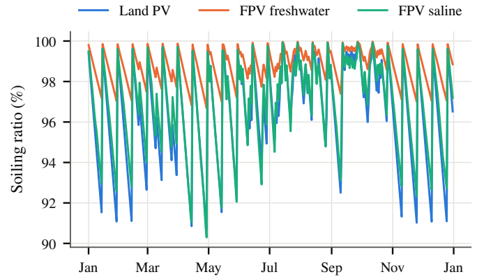
Fig. 6. Daily soiling ratio with rain cleaning, NaCl deliquescence and 15-day manual cleaning (baseline).
