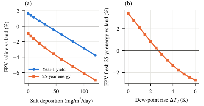
Fig. 9. Break-even thresholds relative to land PV. (a) Saline FPV versus salt-soiling deposition (chloride at baseline). (b) Freshwater FPV 25-year energy versus dew-point rise over water.
