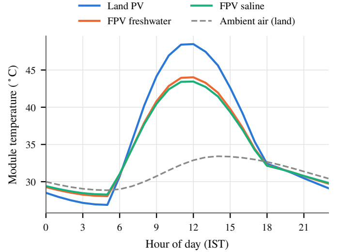
Fig. 3. Mean module temperature by hour of day in May for the three plants, with the site air temperature (baseline parameters).
