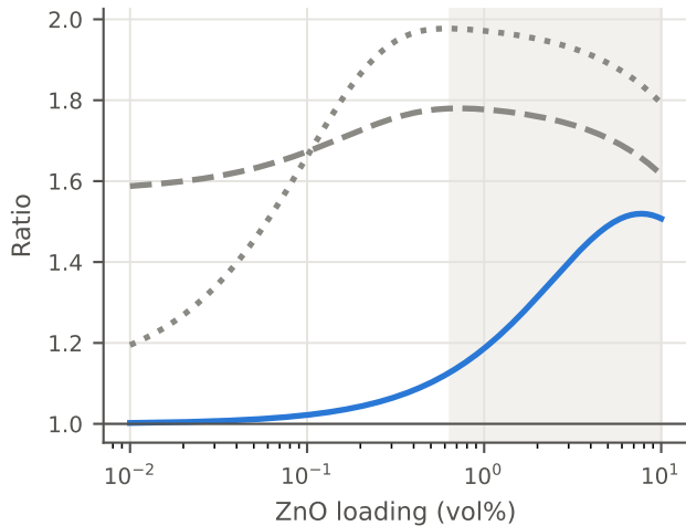
|d_{33}| relative to unfilled film
