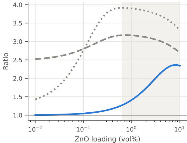
d_{33}g_{33} relative to unfilled film
