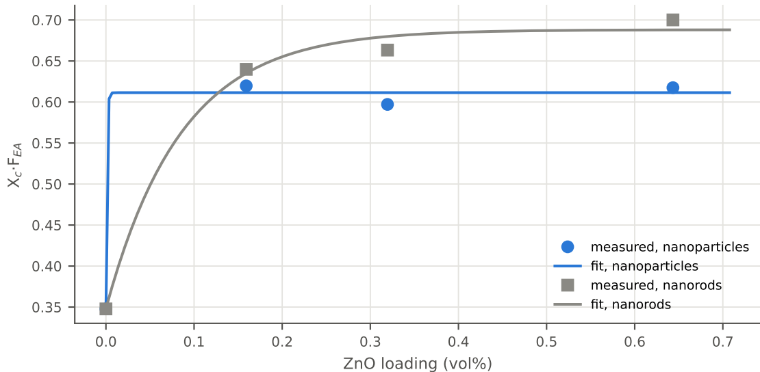
Polar crystalline content X_c F vs ZnO loading (Bagla et al. 2025)
