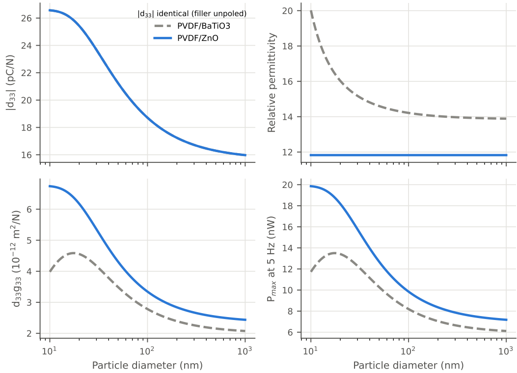
Figure 5: Model-predicted |d_{33}| , permittivity, d_{33}g_{33} and P_{\max} versus particle diameter at 5 vol%, with nucleation tied to interphase volume (Eq. 16; t = 5 nm, \Delta F = 0.35 , \phi_{i,\text{sat}} = 0.05 ). Interphase permittivity: \varepsilon_i = \varepsilon_m for ZnO, \varepsilon_i = 30 for BaTiO 3 .
