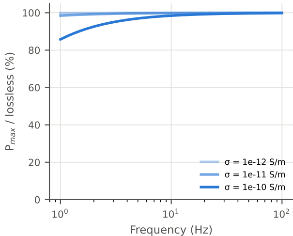
PVDF/ZnO: power retained
