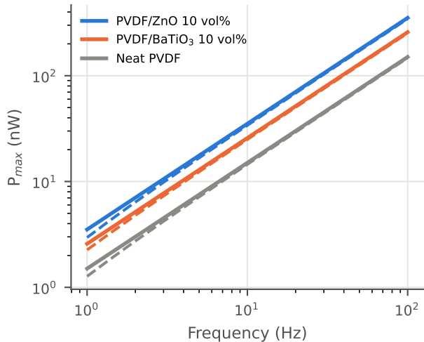
Matched-load power (solid: lossless)
