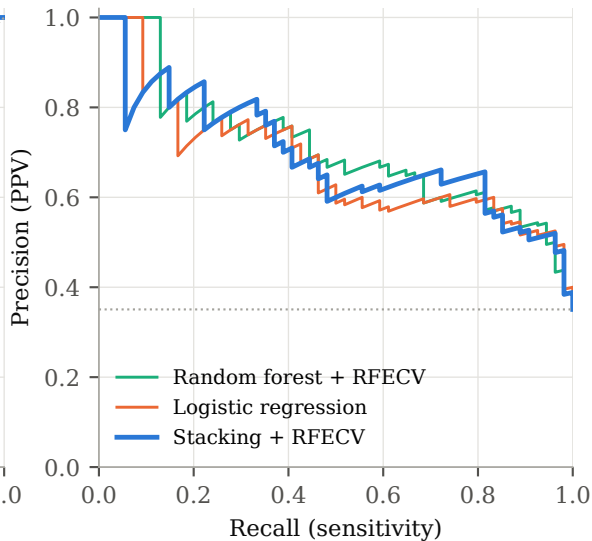
(b) Precision-recall
