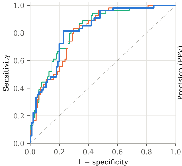
(a) ROC
