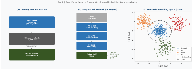
Fig. 2. Deep kernel training: (a) data pipeline; (b) network; (c) t-SNE embedding showing nominal (blue), FDI (red), replay (orange), DoS (green) clusters and detection boundary \gamma_{th}=3.84 (dashed).
