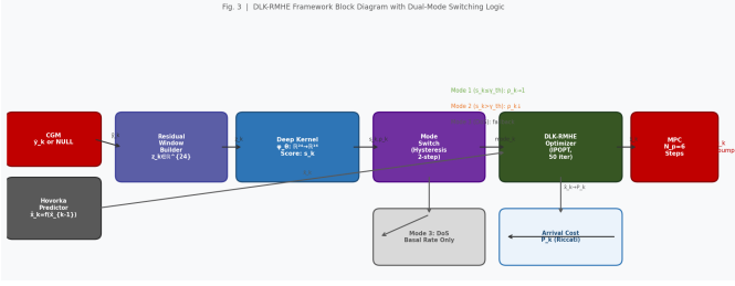
Fig. 3. DLK-RMHE block diagram with dual-mode switching logic.
