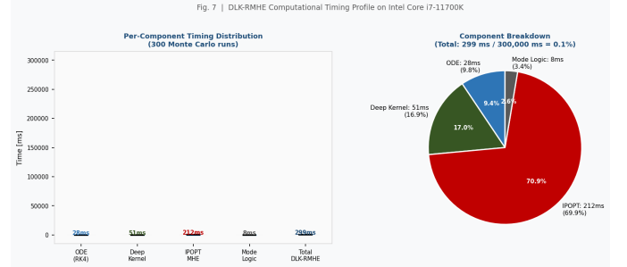
Fig. 7. (Left) Per-component timing violin plots over 300 Monte Carlo runs. (Right) Component breakdown pie chart.
