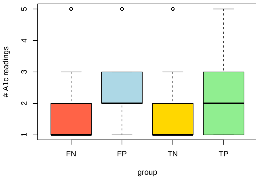
n_a1c by TP/TN/FP/FN
