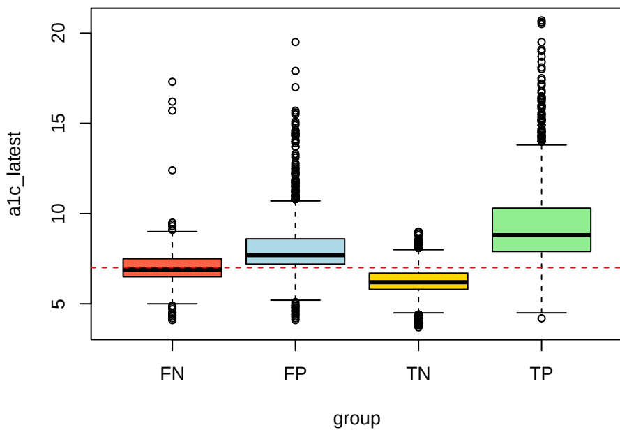
a1c_latest by TP/TN/FP/FN
