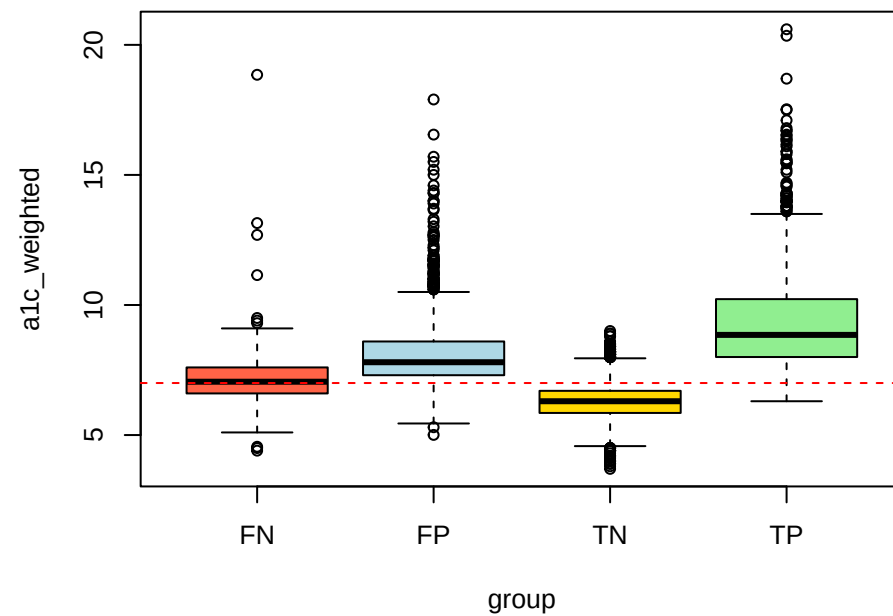
a1c_weighted by TP/TN/FP/FN
