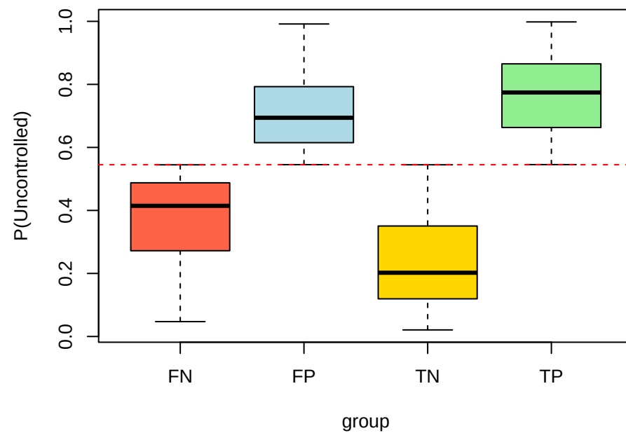
GLM+wt predicted prob by group
