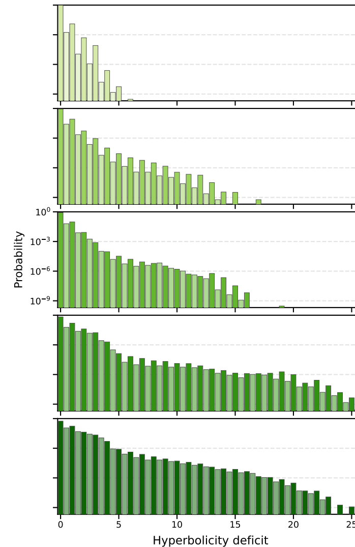
Four-point hyperbolicity
