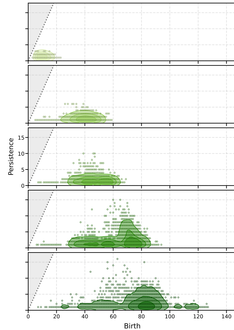
Four-point persistence
