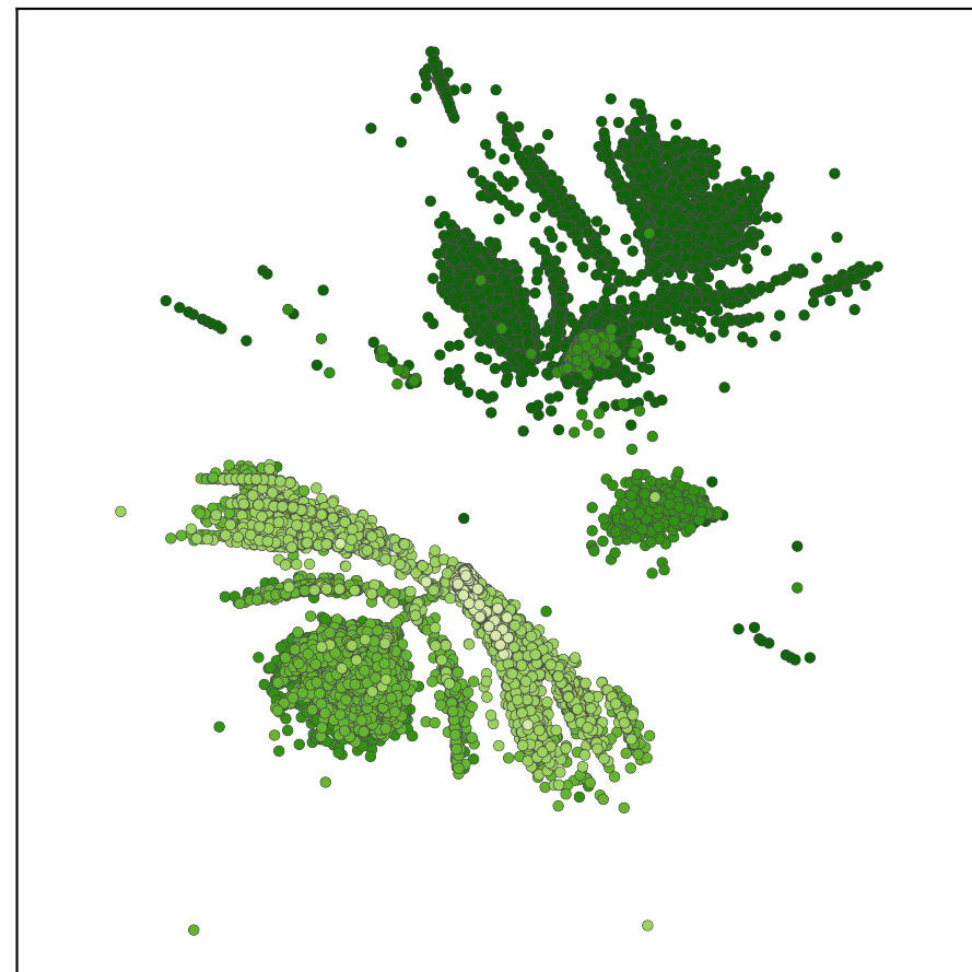
Metric MDS
